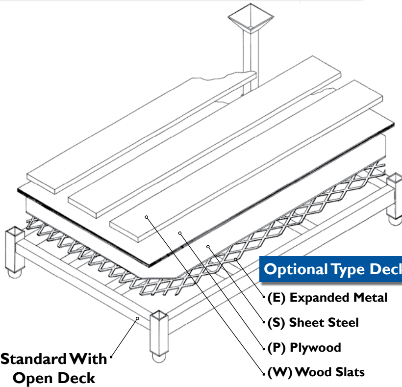
Base Frame Type 808
