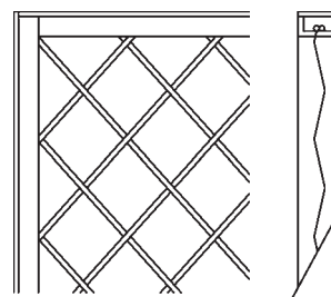
1/2" x 1" x 1/8" channel frame with 1/8" x 1" flat bar cap.
