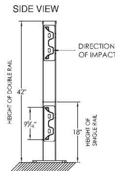
JESCOGARD® Economy Rail Layout
