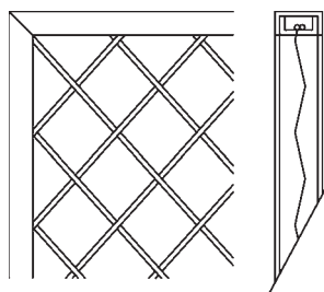
1/2" x 1" x 1/8" channel frame with 5/8" x 1 1/4" x 1/8" channel cap.
