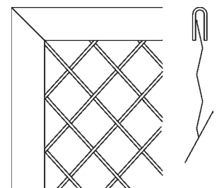
1 1/2" x 16 gauge U-edging with 2" reveal.
