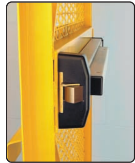
Full width panic bars enable easy exit even in emergency situations. Cylinder lock on front.
