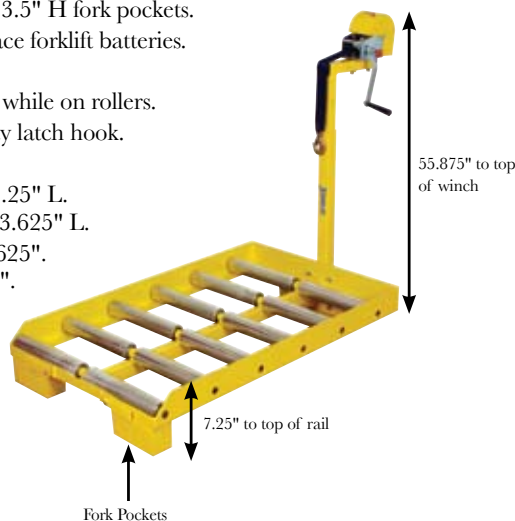
OVERALL DIMENSIONS
